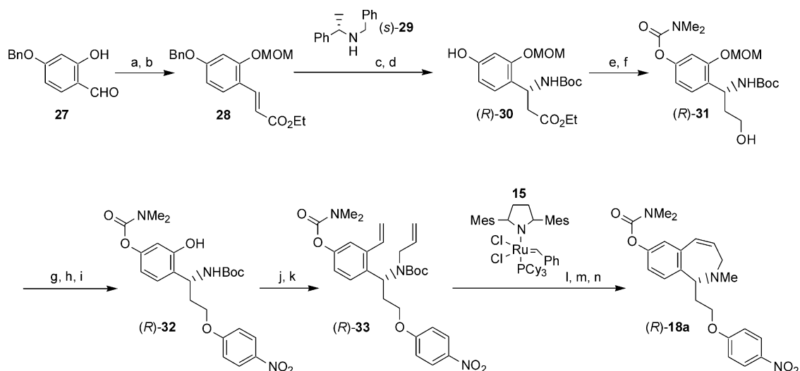
Scheme 4. Reagents and conditions: (a) MOMCl, i -Pr 2 NEt, CH 2 Cl 2 , 0 °C, 79%; (b) (EtO) 2 P(O)CH 2 CO 2 Et, NaH, THF, 0 °C, 99%; (c) (i) ( S )- 29 , n -BuLi, THF, −78 °C; (ii) H 2 , 20% Pd(OH) 2 /C, MeOH–H 2 O–AcOH (20:2:1), rt, 67% (two steps); (d) Boc 2 O, Et 3 N, MeOH, rt, 97%; (e) Me 2 N–COCl, K 2 CO 3 , DMF, rt, 97%; (f) LiAlH 4 , THF, −50 to 0 °C, 82%; (g) p -nitrophenol, DEAD, PPh 3 , THF, rt; (h) concd HCl, MeOH, rt, 68% (two steps); (i) Boc 2 O, Et 3 N, MeOH, rt, 85%; (j) (i) Tf 2 O, py, CH 2 Cl 2 , 0 °C; (ii) (CH 2 =CH)( n -Bu) 3 Sn, Pd(PPh 3 ) 4 , LiCl, dioxane, 100 °C, 86% (two steps); (k) allyl bromide, NaH, DMF, 0 °C to rt, 86%; (l) 15 (10 mol%), CH 2 Cl 2 (15 mM), 45 °C, 96%; (m) 2 N HCl–AcOEt, rt, 96%; (n) (i) 37% HCHO aq., HCO 2 H, 80 °C, 78%.
