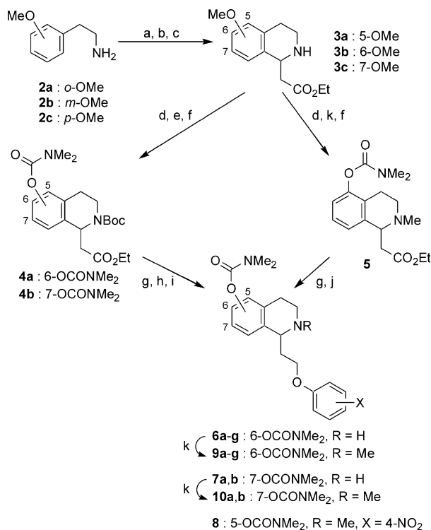
Scheme 1. Reagents and conditions: (a) ethyl malonyl chloride, \text{K}_2\text{CO}_3 , \text{CH}_2\text{Cl}_2 , 0^\circ\text{C} ; (b) \text{POCl}_3 or PPE, 80^\circ\text{C} ; (c) \text{H}_2 , \text{PtO}_2 , \text{AcOH} , rt; (d) \text{BBr}_3 , \text{CH}_2\text{Cl}_2 , -78^\circ\text{C} to rt; (e) \text{Boc}_2\text{O} , THF, rt; (f) \text{Me}_2\text{NCOCl} , \text{K}_2\text{CO}_3 , DMF, rt; (g) \text{LiAlH}_4 , THF, -78 to 0^\circ\text{C} ; (h) phenol, DEAD, \text{PPh}_3 , THF, rt; (i) 2N \text{HCl} – \text{AcOEt} , rt; (j) 1-fluoro-4-nitrobenzene, NaH, DMF; (k) 37% \text{HCHO} aq, \text{HCO}_2\text{H} , 80^\circ\text{C} .
