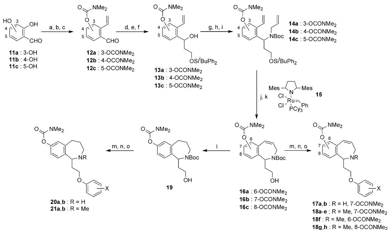
Scheme 2. Reagents and conditions: (a) Me 2 NCOCl, NaH, DMF, rt or Me 2 NCOCl, py, CH 2 Cl 2 , rt; (b) Tf 2 O, py, CH 2 Cl 2 , 0 °C; (c) (CH 2 =CH)( n -Bu) 3 Sn, Pd(PPh 3 ) 4 , LiCl, dioxane, 100 °C; (d) AcOEt, LDA, THF, −78 °C; (e) LiBH 4 , THF, rt; (f) t -BuPh 2 SiCl, imidazole, DMF, rt; (g) CBr 4 , PPh 3 , CH 2 Cl 2 , rt; (h) allylamine, CH 3 CN, rt; (i) Boc 2 O, Et 3 N, THF, 50 °C; (j) 15 (10 mol%), CH 2 Cl 2 , 45 °C; (k) TBAF, THF, rt; (l) H 2 , Pd/C, MeOH, rt; (m) phenol, DEAD, PPh 3 , THF, rt; (n) 2 N HCl–EtOAc, rt; (o) 37% HCHO aq, HCO 2 H, 80 °C.
