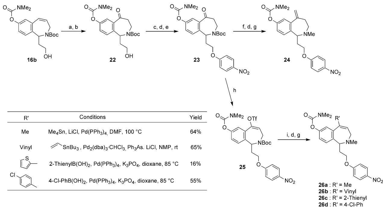
Scheme 3. Reagents and conditions: (a) BH 3 , THF, 0 °C to rt then NaBO 3 , 0 °C to rt; (b) MnO 2 , CH 2 Cl 2 , rt; (c) p -nitrophenol, DEAD, PPh 3 , THF, rt; (d) 2N HCl–AcOEt, rt; (e) Boc 2 O, Et 3 N, THF, rt; (f) Ph 3 P + CH 3 Br − , t -BuOK, benzene, 80 °C; (g) 37% HCHO aq., HCO 2 H, 80 °C; (h) 2-(5-Cl-Py)NTf 2 , LHMDS, THF, −78 °C; (i) see scheme.
